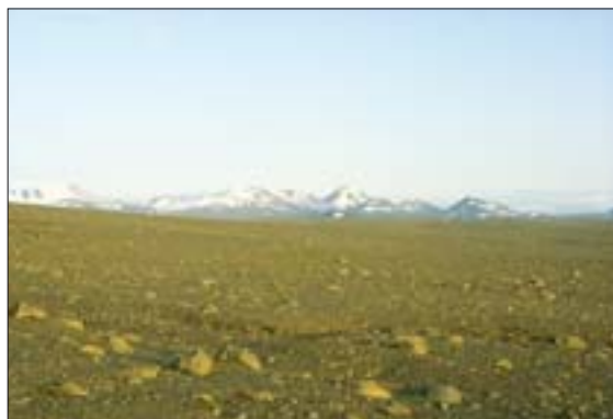
Melur. A glacial till with stony surface and not much loose sand.
