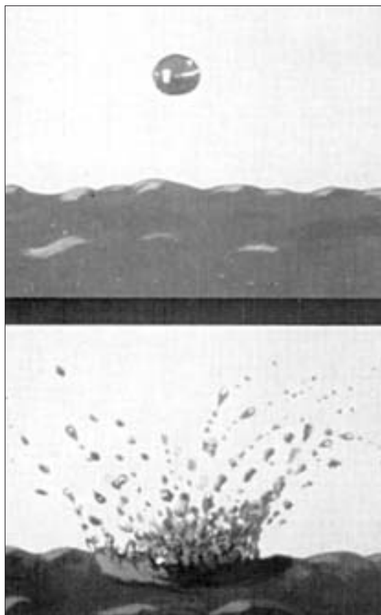
Rain-splash detaches soil particles on the surface. High-speed pictures. (US-SCS).
