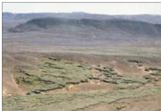
Severely degraded land, not suitable for grazing. Rapid erosion is taking place along the edges of the remaining vegetation (rofabards).
